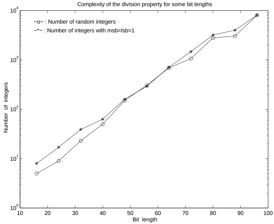
Figure 1: Experimental results. The line \circ describes the number of random k -bit integers, and the line \star describes the number of random k -bit integers with the first and last bits set to '1'.
