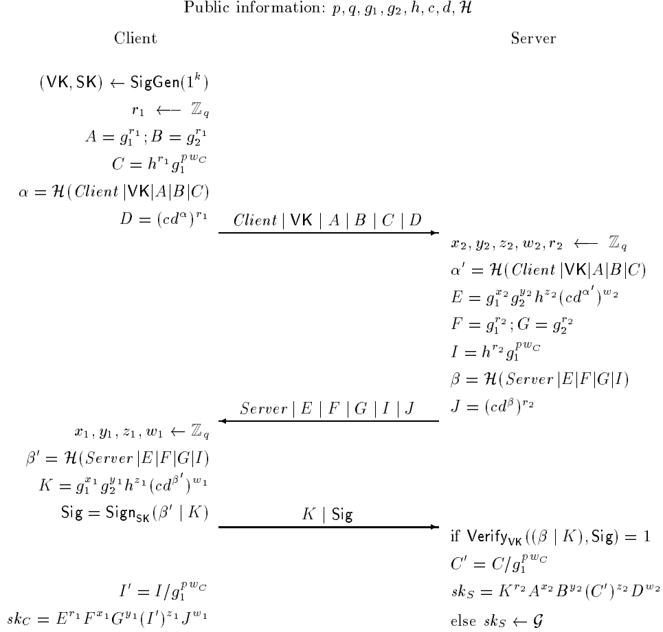
Fig. 1. The protocol for password-AKE. See text for details.
