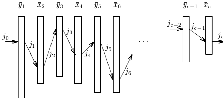
Figure 1: Demonstration of GInd . Alice holds \hat{x} = \bar{x}_2, \bar{x}_4, \dots, \bar{x}_c and Bob holds \hat{y} = \bar{y}_1, \bar{y}_3, \dots, \bar{y}_{c-1} . The outcome is x_c[y_{c-1}[\dots[x_2[y_1[j_0]]]\dots]] shared between Alice and Bob. The intermediate indices j_1, \dots, j_c are not revealed to any of the parties.
