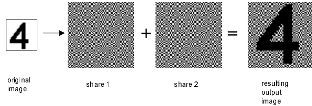
Fig. 2. Naor-Shamir visual cryptography example where every original pixel is split into four sub-pixels.
