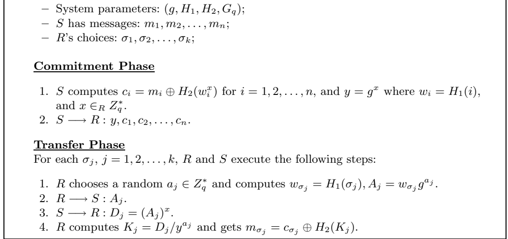
Fig. 3. Adpt-OT _n^k : Adaptive OT _n^k
