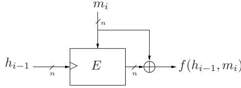
Figure 1: The Matyas-Meyer-Oseas (MMO) compression function [8]. E: \{0,1\}^n \times \{0,1\}^n \rightarrow \{0,1\}^n is a block cipher; the hatch mark denotes the location of the key. Iterating this compression function results in a provably-secure hash function [2], however notice that the above compression function will be rekeyed each round.
