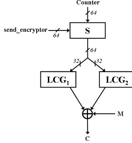
Figure 5: The ICC Mode of Operation: 64 bits are generated by enciphering a counter under the sender’s blockcipher key. The first 32 are sent to LCG_1 and the other 32 to LCG_2 . The LCG’s are iterated 100 times and their lowest bytes are XORed to produce an encryption pad which is XORed with the message M to produce the ciphertext C .
