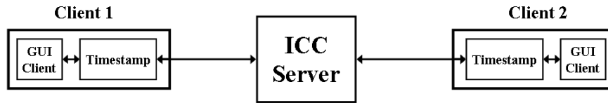
Figure 2: The ICC configuration: clients communicate through a timestamp process which records the arrival-time of incoming moves and computes the elapsed time for a player’s move before transmitting it to the server. The timestamp process can be run on a different machine, but it is most often on the local machine. Some clients have the timestamp process built-in; this is the case with the Blitzin Windows client but not with any of the Unix clients.
