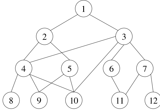
Fig. 1. Example of a Hasse diagram
