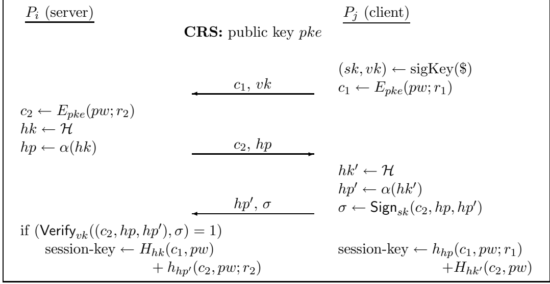
Figure 3: The core of the KOY/GL protocols.
