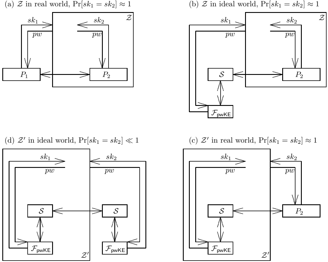
Figure 8: The four cases in the proof of Theorem 3.
