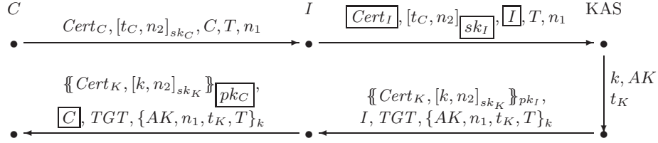
Fig. 2. Message Flow in the Man-In-The-Middle Attack on PKINIT-26
