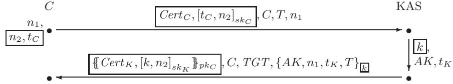
Fig. 1. Message Flow in the Traditional AS Exchange and in PKINIT-26
