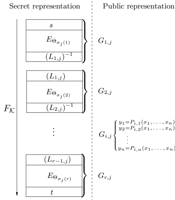
Figure 1: A traceable block cipher
