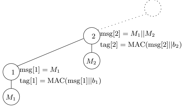
Figure 4: A tree-based description of the computation of authentication tags in ReMAC
