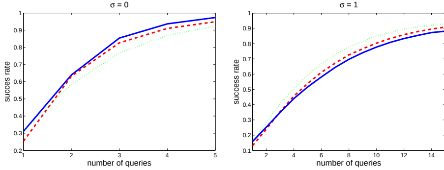
Fig. 4. 1 st -order success rates in function of the number of queries for the leakages functions corresponding to Z_1 (solid line), Z_2 (dashed line) and Z_3 (dotted line).
