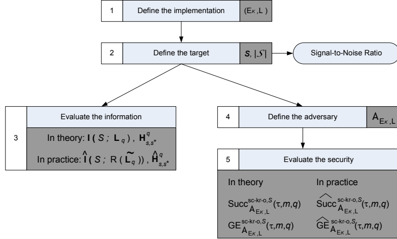
Fig. 5. Evaluation methodology for side-channel attacks.
