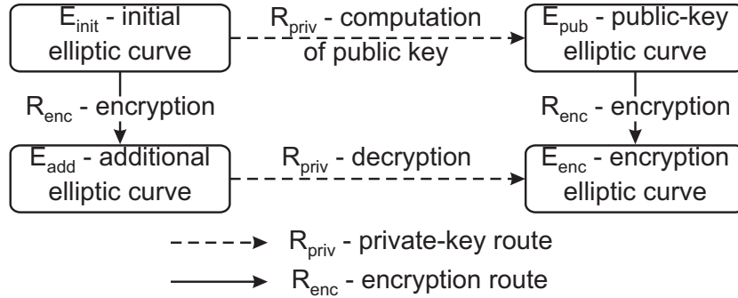
Fig. 3. Public-key encryption scheme on isogeny star.
