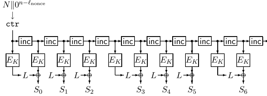
Figure 3: Illustration of the keystream generation algorithm. This example uses w = 3 and outputs l = 7 blocks of keystream S = (S_0, \dots, S_6) . This S is used in both encryption and decryption. The mask L is updated after generating w blocks of keystream. The counter ctr is incremented for l + \lceil l/w \rceil = 10 times, and there are 10 blockcipher invocations.
