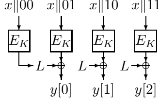
Figure 1: Example illustration of F . In this example, w = 3 , \omega = 1 + \lfloor \log_2 w \rfloor = 2 , and F : \{0, 1\}^k \times \{0, 1\}^{n-2} \rightarrow (\{0, 1\}^n)^3 where F_K(x) = (y[0], y[1], y[2]) . Here x \in \{0, 1\}^{n-2} , y[0] = L \oplus E_K(x||01) , y[1] = L \oplus E_K(x||10) , y[2] = L \oplus E_K(x||11) , where L = E_K(x||00) .
