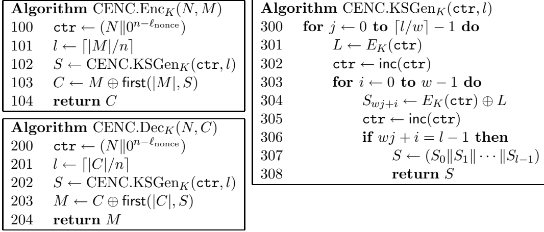
Figure 2: Definition of the encryption algorithm CENC.Enc (left top), the decryption algorithm CENC.Dec (left bottom), and the keystream generation algorithm CENC.KSGen (right), which is used in both encryption and decryption.
