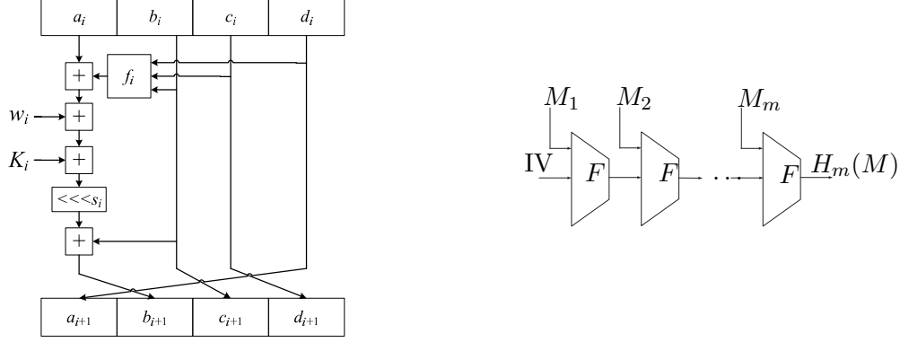
Figure 1: One round of Feistel ladder for MD5 and the Merkle-Damgård construction.
