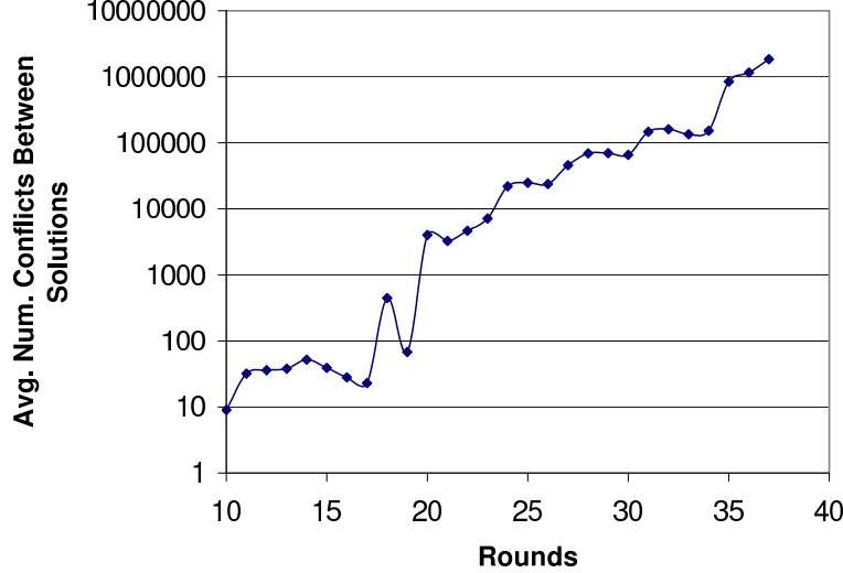
Figure 5: Number of conflicts for finding 10000 solutions in reduced-round MD5.
