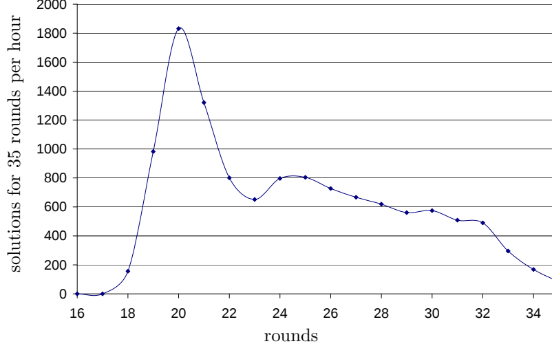
Figure 4: Normalized performance of SATELITEGTI on reduced-round SHA0 (axis x —number of rounds; y —“yield”, defined here as the number of solutions for 35-round differential per hour).
