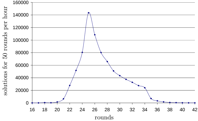
Figure 3: Normalized performance of SATELITEGTI on reduced-round MD5 (axis x —number of rounds; y —“yield”, defined here as the number of solutions for 50-round differential per hour).
