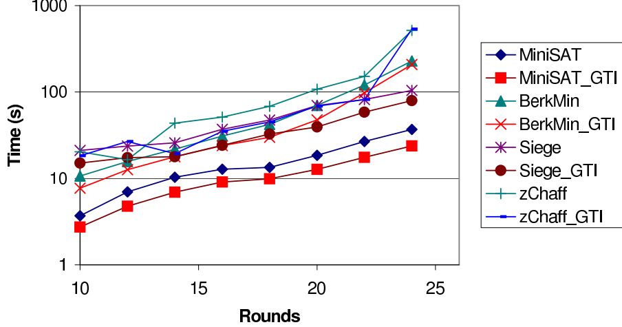
Figure 2: Comparison of Different Solvers on MD5 Instances.
