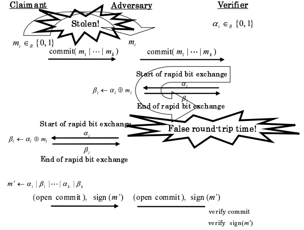
Fig. 4: Replay attack using a stolen nonce on the distance bounding with bidirectional communication [5]. The adversary makes up the false round-trip time with the stolen nonce. The adversary successfully deceives the verifier without claimant's private key for digital signatures.
