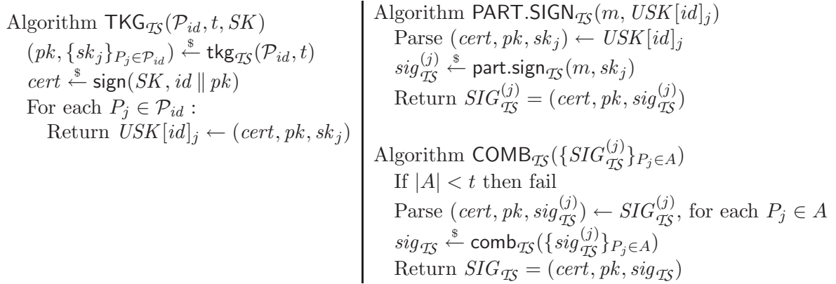
Figure 6: Generic construction of identity-based TS.
