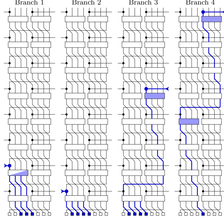
Fig. 3. High-level path used to find near-collisions in FORK-256. Thick lines show the propagation of differences. Q -structures for which microcollisions have to be found are grayed out.
