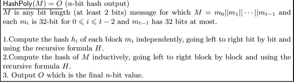
Fig. 1. Hashing with Polynomials.
