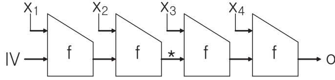
Fig. 3. Merkle-Damgård Construction in case of 4 block-message. IV is the initial value.
