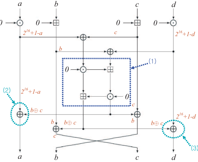
Fig. 4. Analysis of Round Function of IDEA
