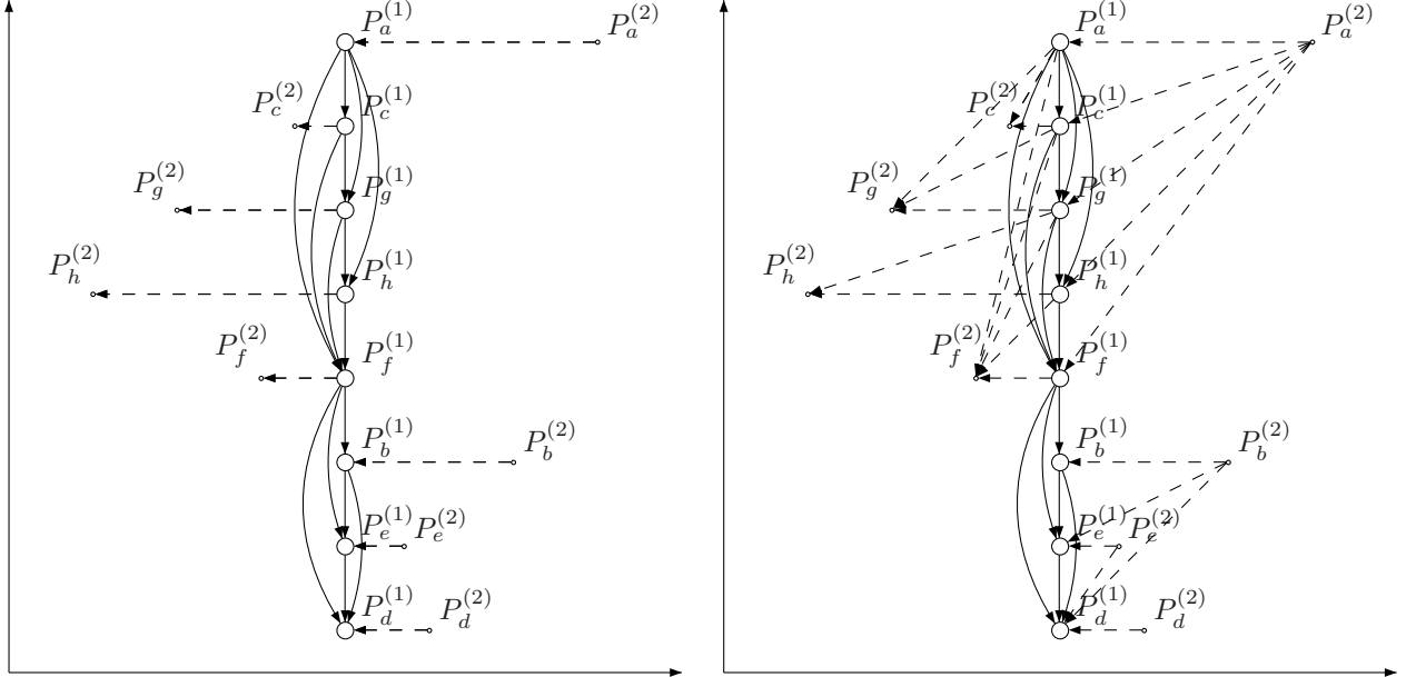
Figure 11: New edges added by our algorithm in steps 7. and 8.
