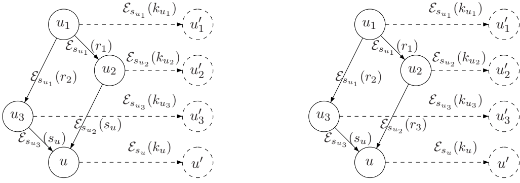
Figure 4: The left hand side illustrates \mathbf{Exp1}_u^3 while the right hand side illustrates \mathbf{Exp1}_u^4 .
