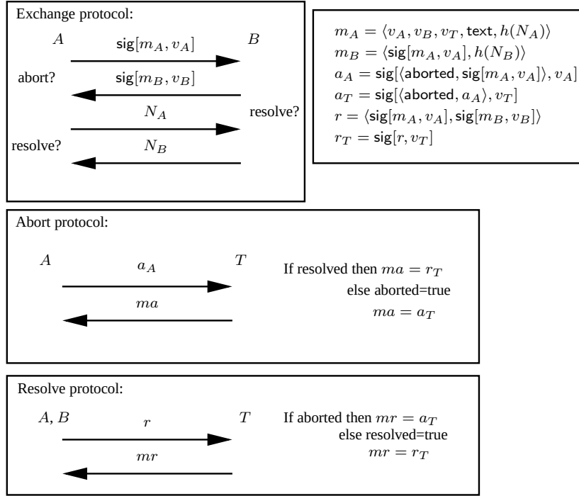
Fig. 1. The ASW Protocol. We indicate where during the execution of the Exchange protocol parties can choose to run the Abort or the Resolve subprotocols.
