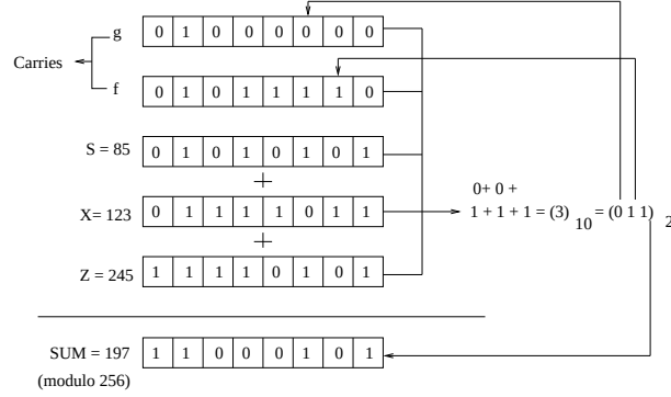
Fig. 2. An example showing how the carries are generated when three 8-bit variables S = 85 , X = 123 and Z = 245 are added
