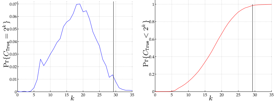
Fig. 3. Probability density (left) and cumulative (right) functions of the time C_{\text{True}} in logarithmical form ( k = \log_2 C_{\text{True}} ). The scenario is N = 64 , \mathcal{M}_{\text{g}} and 2000 samples.
