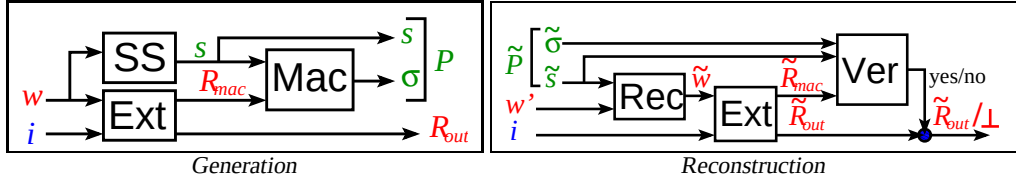
Fig. 1. Construction of Robust Fuzzy Extractor
