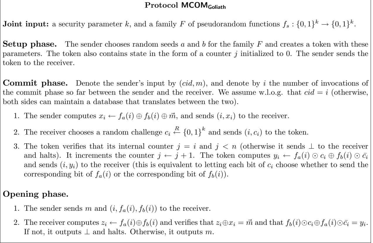
Figure 6: Protocol \text{MCOM}_{\text{Goliath}} .
