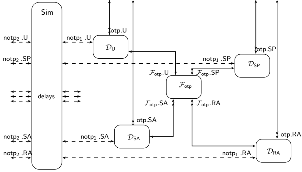
Fig. 2. OTP simulator
