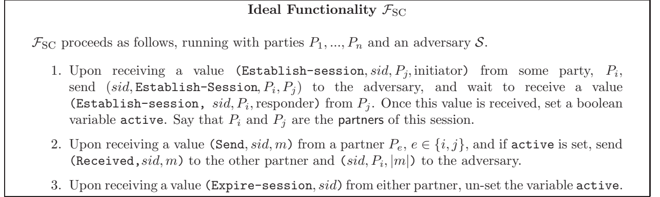
Figure 1: The Secure Channels functionality, \mathcal{F}_{SC}
