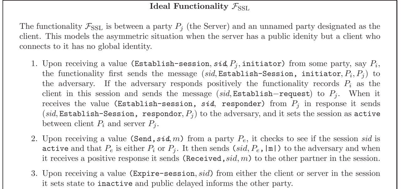
Figure 2: The SSL functionality, \mathcal{F}_{SSL}
