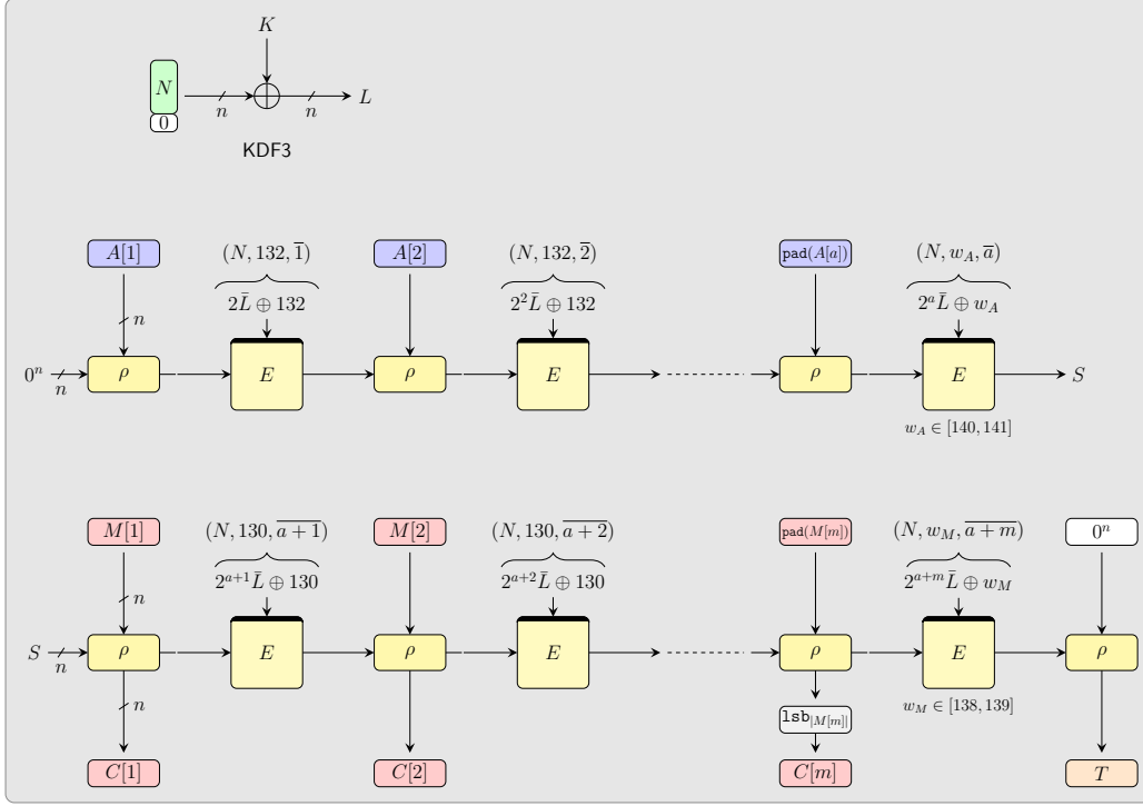
Figure 9: Remus-N with ICE3 (Remus-N3). (Top) Key derivation (computing (2^D L[1]) \parallel (B \oplus L[2]) , we use the \bar{L} notation to represent the fact that the multiplication is only done on L[1] , the first k-8 bits of L ). (Middle) Processing of AD (Bottom) Encryption. The domain separation B being of 8 bits only, \oplus B is to be interpreted as \oplus 0^{120} \parallel B .
