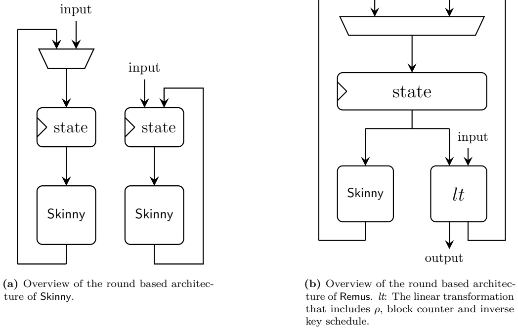
Figure 18: Expected architectures for Skinny and Remus
