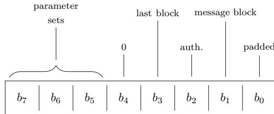
Figure 17: Domain separation when using the tweakable block cipher
