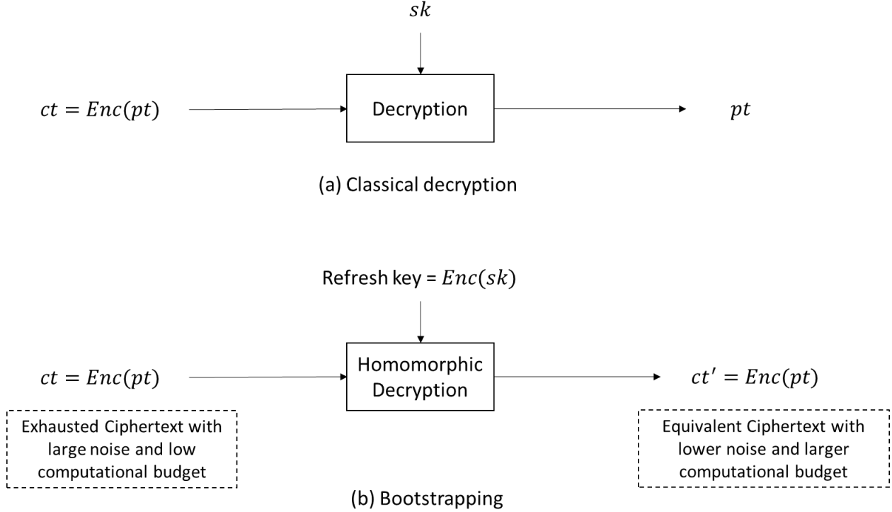
Figure 1: (a) Classical decryption vs (b) homomorphic decryption or bootstrapping. A ciphertext is generated as an encryption ( \text{Enc} ) of a certain plaintext message pt under a certain secret key sk . The refreshing or bootstrapping key is an encryption of the sk and is supposed to be made publicly available to the evaluator under the circular security assumption.
